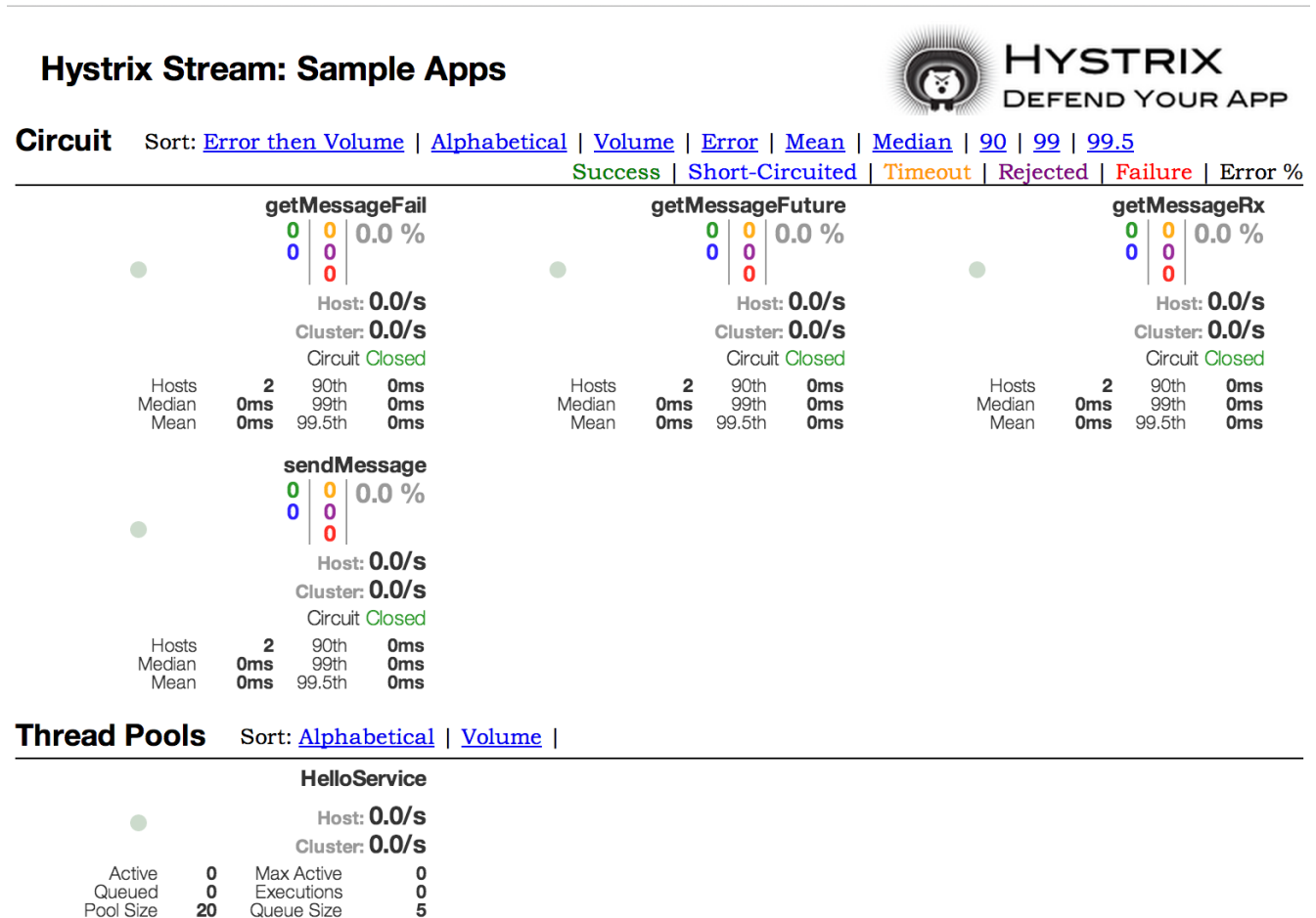
Figure 1. Microservice Graph
